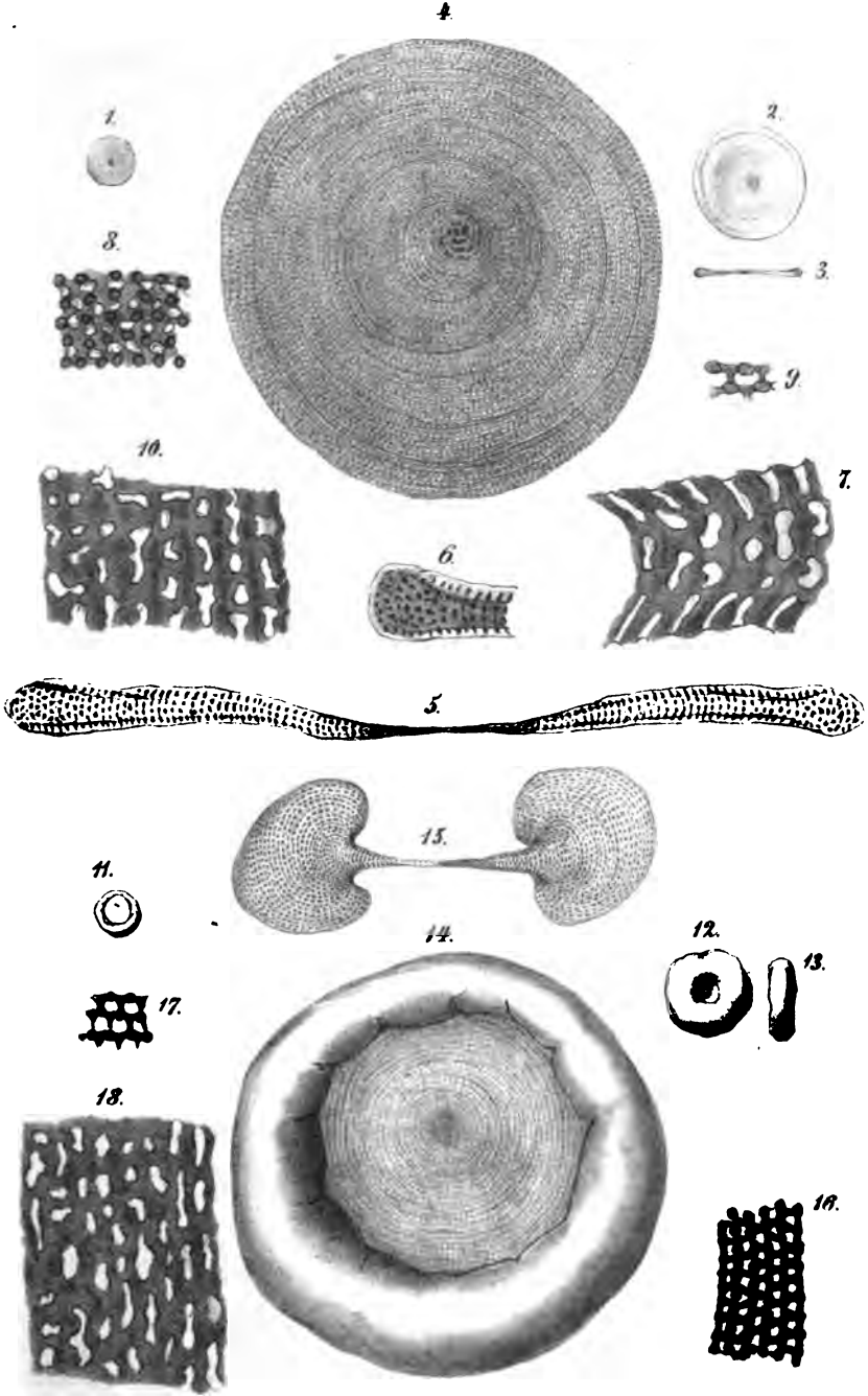
1-10 Orbitolites praecursor Gumb.
